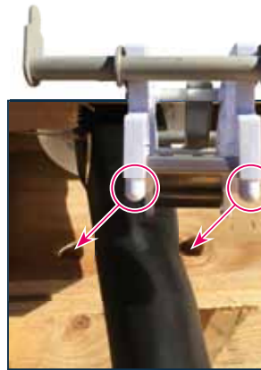
3. Insert the tap base pins in the pallet openings
