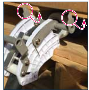
4. Position the tap top pins in the pallet openings
